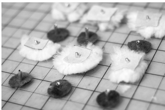
3. Cut a hole in the middle of the weatherstrip and sheepskin. Attach bookbinding screw into them.
